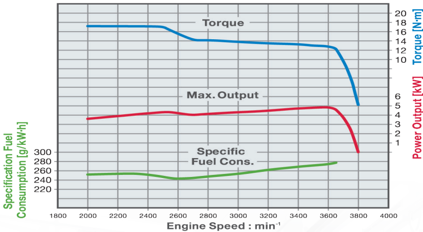
PERFORMANCE CURVES L70W6
