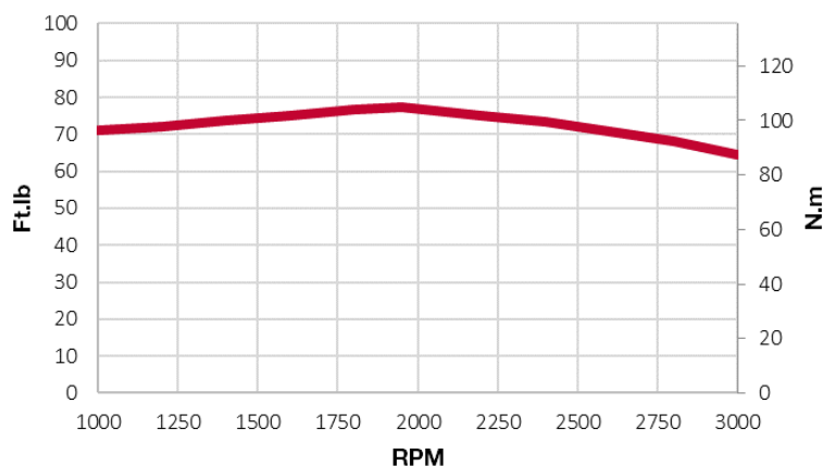
TORQUE
