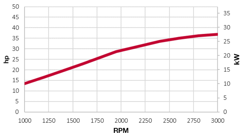
POWER
