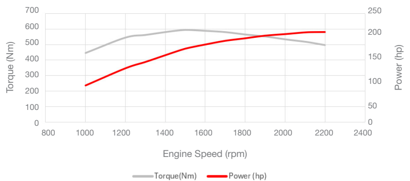
Performance Curves
